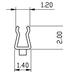
C-C SECTION
