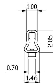
C-C SECTION
