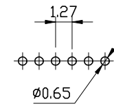
P.C. Board Hole Layout
