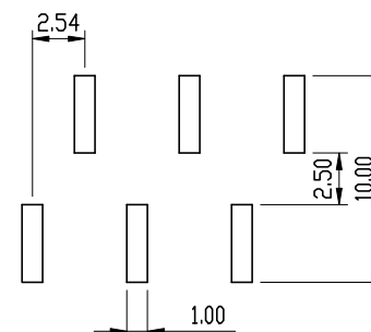
P.C. Board SMT Layout
