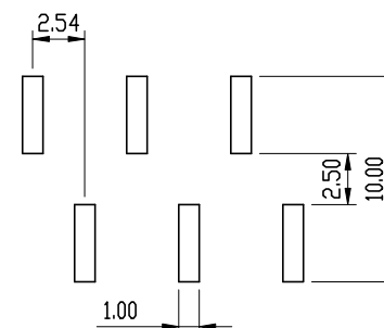
P.C. Board SMT Layout
