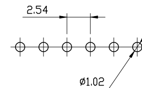
P.C. Board Hole Layout
