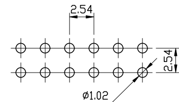
P.C. Board Hole Layout
