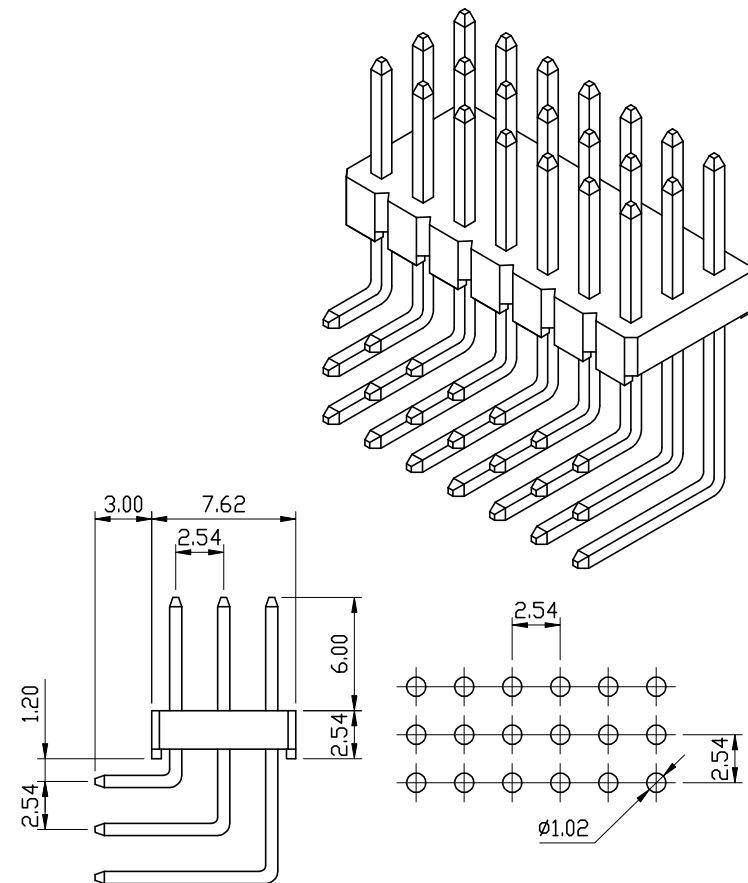
P.C. Board Hole Layout
