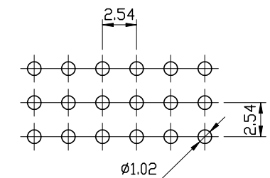
P.C. Board Hole Layout
